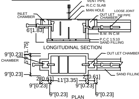
SEPTIC TANK:
