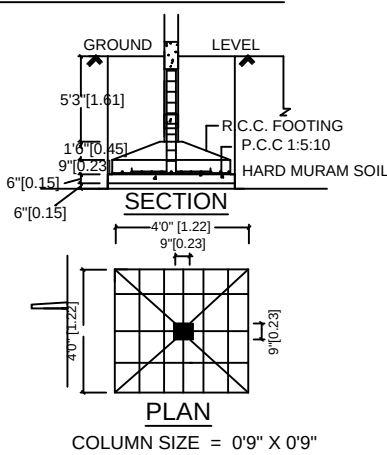
FOUNDATION DETAILS
