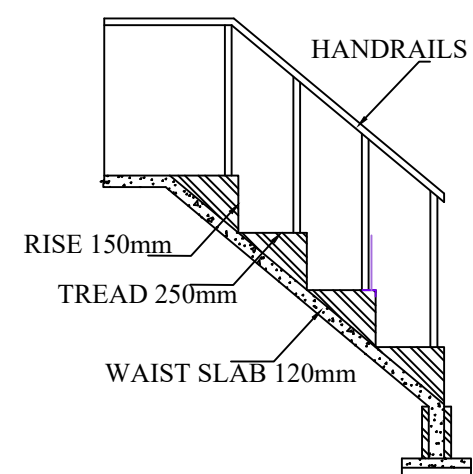
STAIRCASE DETAILS
