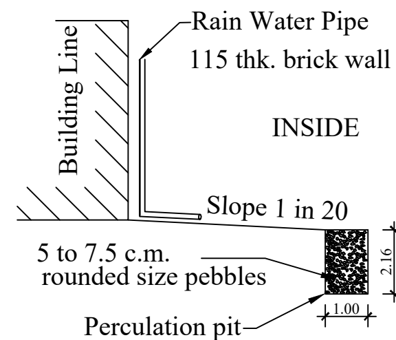
RAIN WATER HARVESTING PERCOLATION PIT
