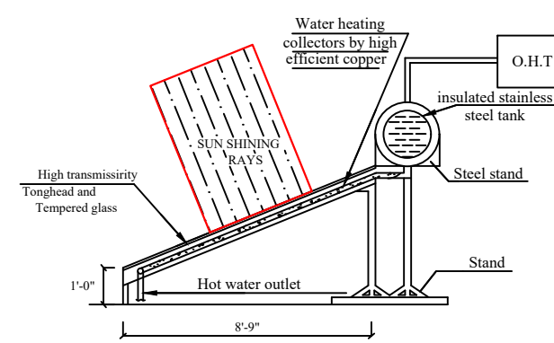
SECTION SOLAR WATER HEATER
