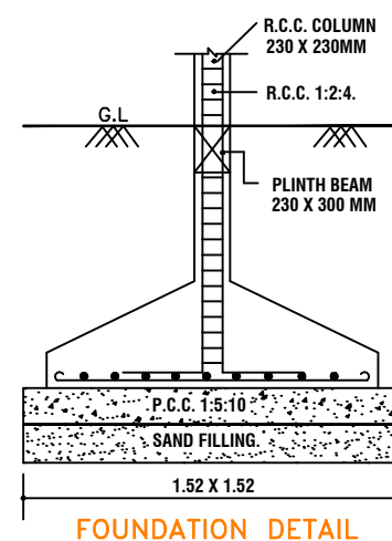
FOUNDATION DETAIL
