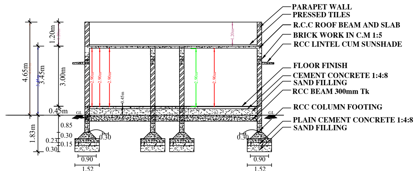
SECTION [A-A]
