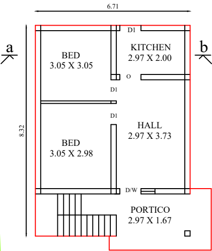
PROPOSED PLAN
