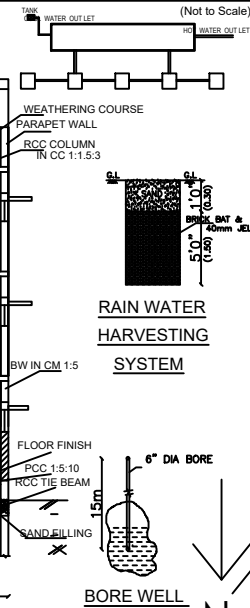
BORE WELL
