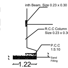
FOUNDATION DETAILS
