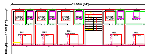
PRO. SECOND FLOOR PLAN
