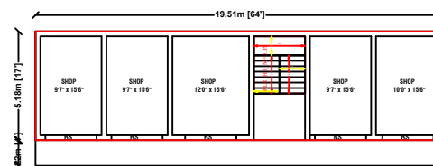
EXG. GROUND FLOOR PLAN
