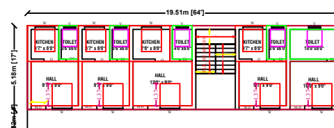
PRO. FIRST FLOOR PLAN
