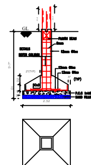
FOUNDATION DETAILS SCALE : 1:50.
