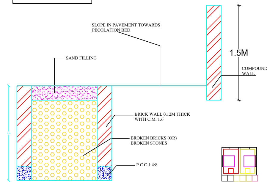
SECTION OF RAIN WATERPERCOLATION BED
