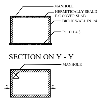
UG - SUMP DETAILED PLAN
