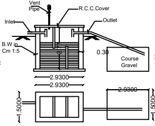
SEPTIC TANK & D-TRENCH DETAILS
