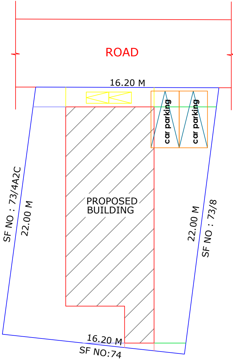
SITE PLAN SALE (1:100)
