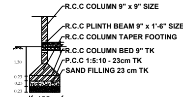
SECTION COLUMN DETAILS PLAN
