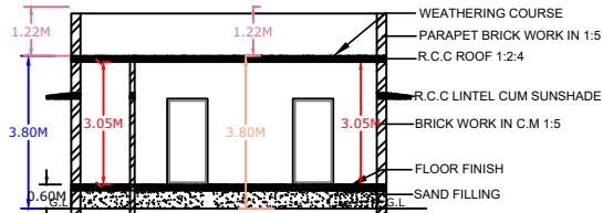
SECTION ON XX
