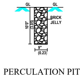
PERCOLATION PIT
