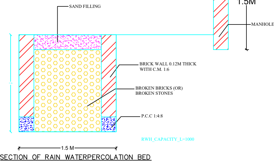
SECTION OF RAIN WATER PERCOLATION BED
