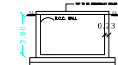
SECTION (SAMPLE)
