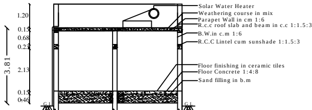
SECTION - "AB "
