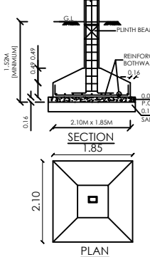
FOUNDATION DETAILS
