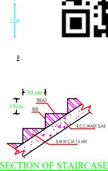
SECTION OF STAIRCASE
