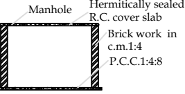
Section On 'Y-Y'
