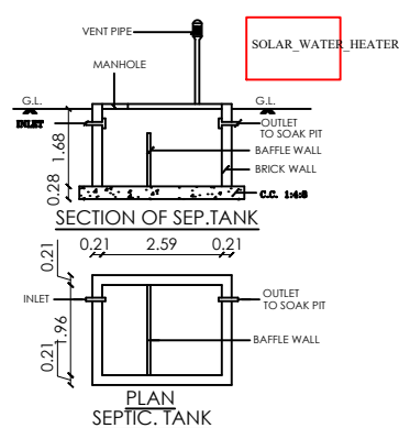
SECTION OF SEP. TANK
