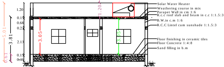
SECTION - "AB "
