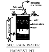
SEC. RAIN WATER HARVEST PIT
