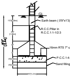
FOUNDATION DETAILS
