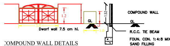
COMPOUND WALL DETAILS
