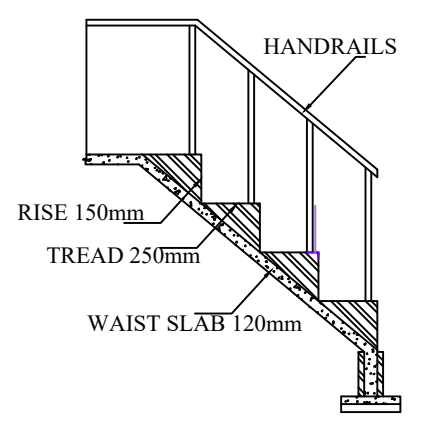
STAIRCASE DETAILS
