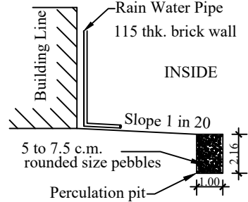
RAIN WATER HARVESTING PERCOLATION PIT
