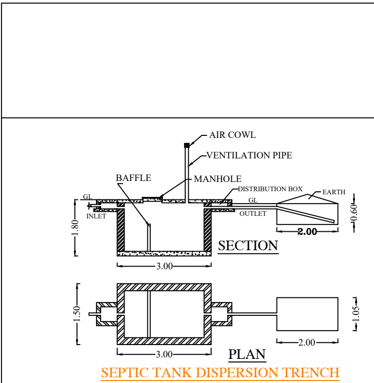
SEPTIC TANK DISPERSION TRENCH
