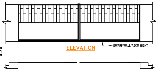
PLAN OF COMPOUND WALL
