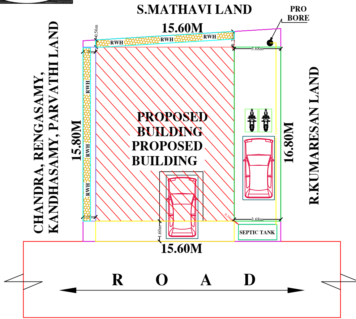
SITE PLAN
