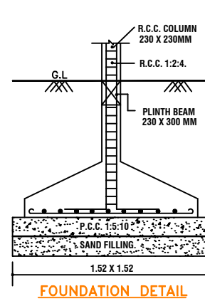
FOUNDATION DETAIL
