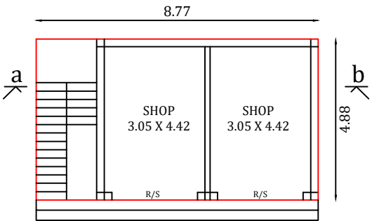
PROPOSED PLAN
