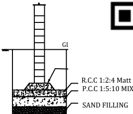
COLUMN DETAILS
