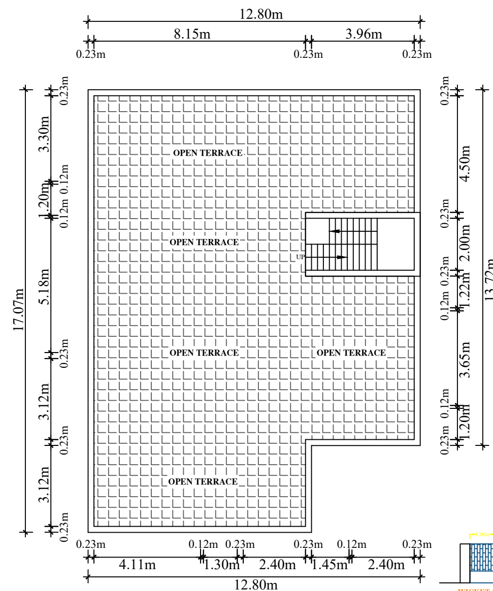
FIRST FLOOR PLAN HEAD ROOM
