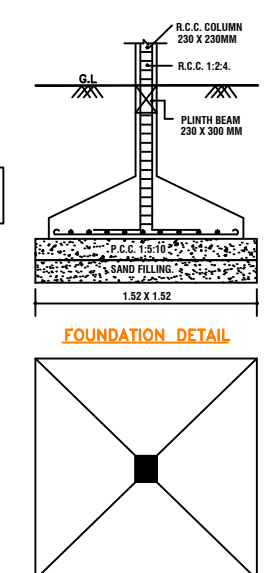
PLAN OF COLUMN FOUNDATION
