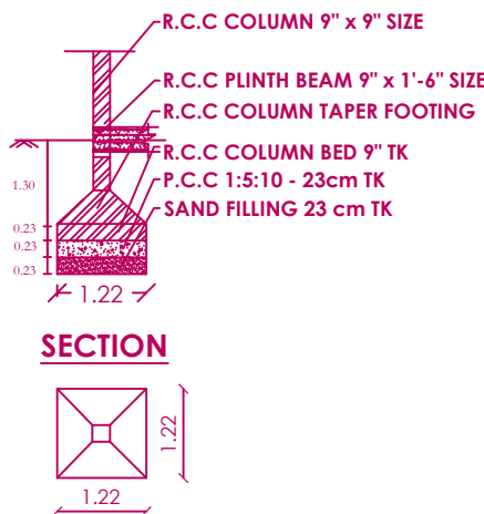
COLUMN DETAILS PLAN
