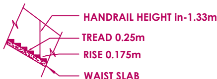
STAIRCASE DETAILS
