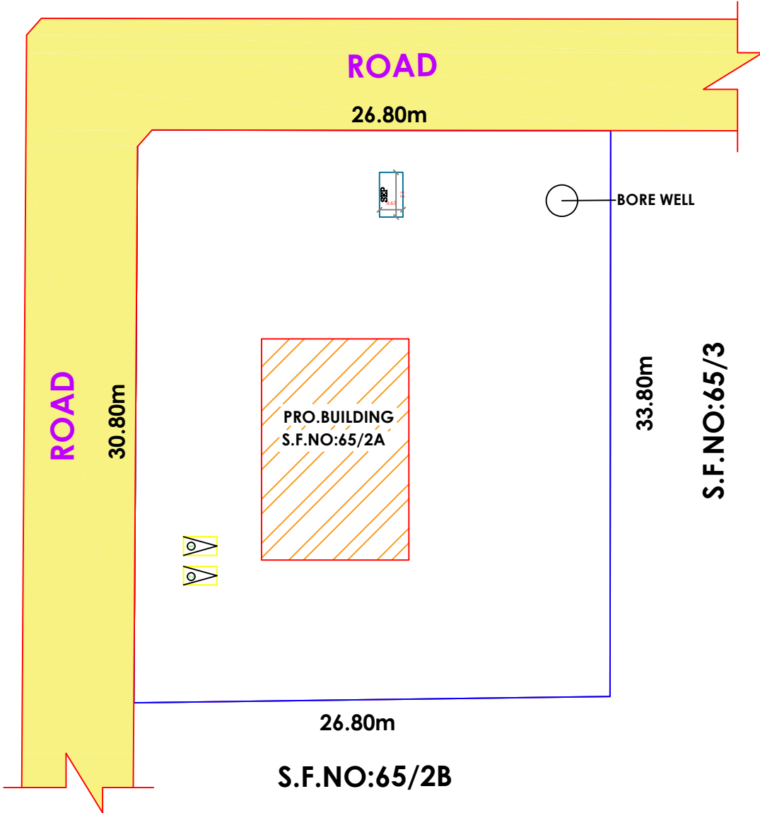
SITE PLAN-SCALE1:200
