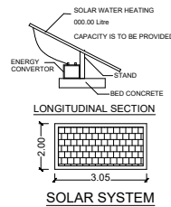
SOLAR SYSTEM
