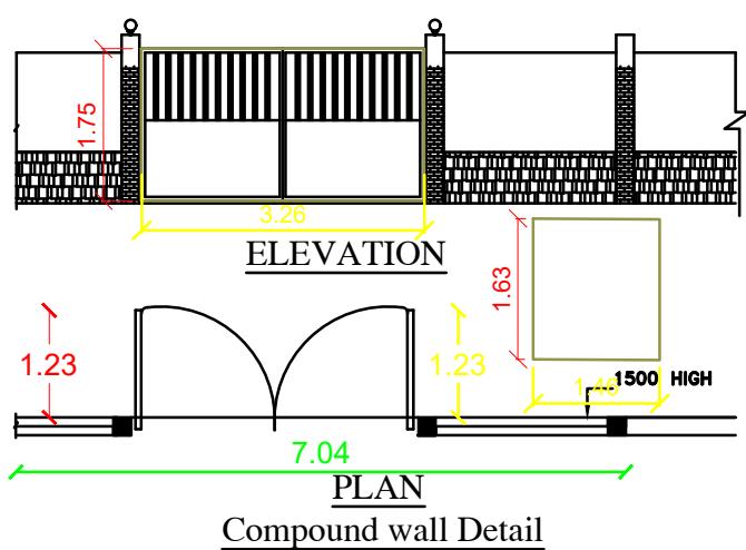
Compound wall Detail
