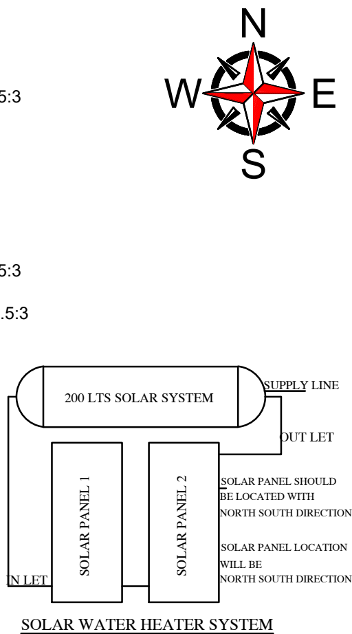
SOLAR WATER HEATER SYSTEM
