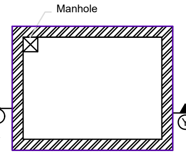
Sump Detail - Plan
