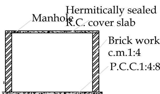
Section On 'Y-Y'
