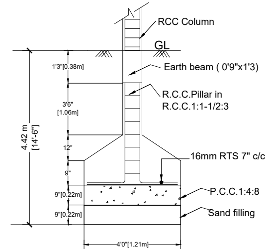
FOUNDATION DETAILS
