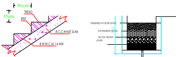
SECTION OF STAIRCASE
