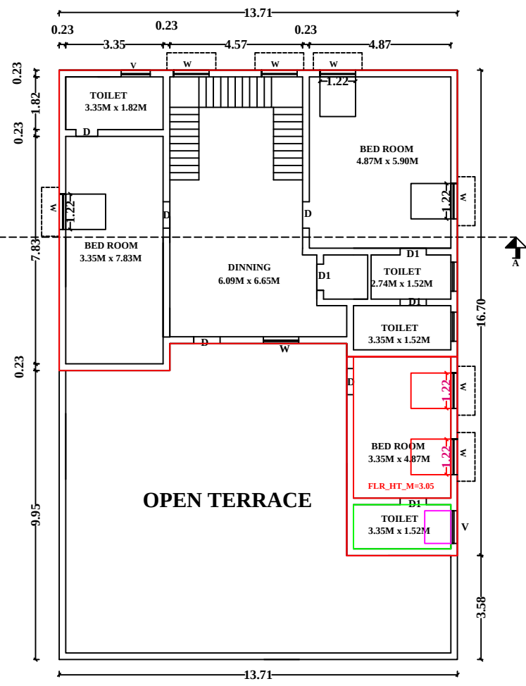
FLOOR-1 PRO.FIRST FLOOR PLAN
