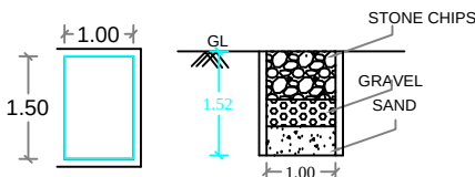
RWH_CAPACITY_L=5000.0 RAIN WATER HARVEST PIT NOT TO SCALE
