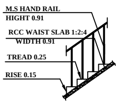
STAIRCASE DETAIL
