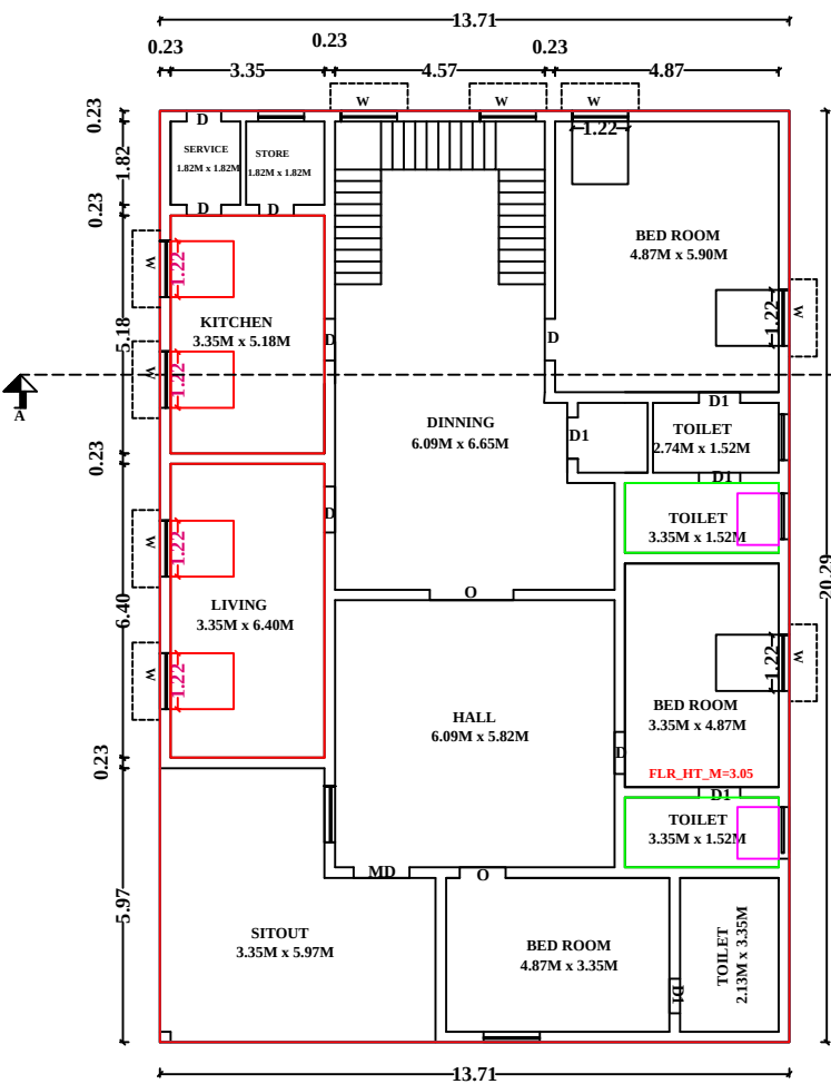
FLOOR-GROUND EXG.GROUND FLOOR PLAN
