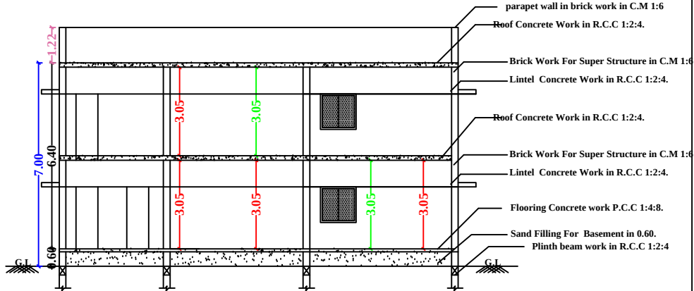
SECTION-AB
