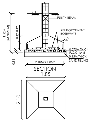
FOUNDATION DETAILS
