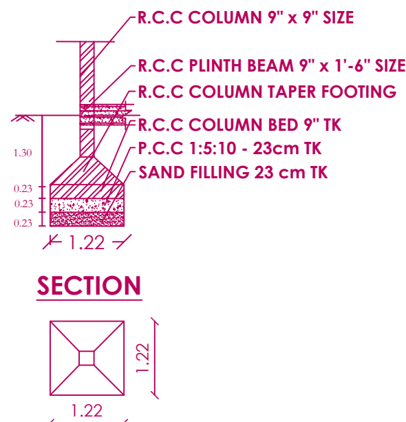
COLUMN DETAILS PLAN
