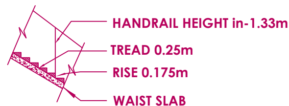
STAIRCASE DETAILS
