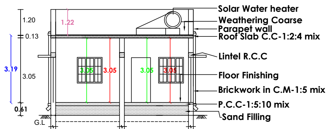
SECTION"AB"
