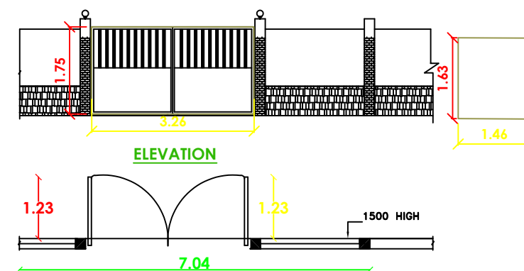
PLAN COMPOUND WALL DETAILS
