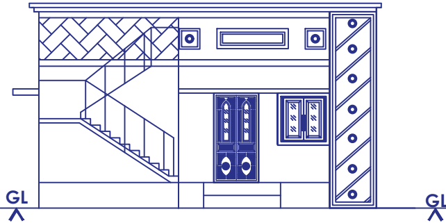
FRONT ELEVATION
