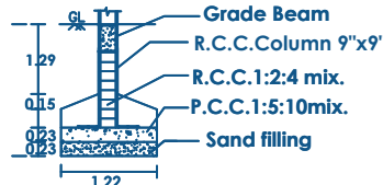
COLUMN DETAILS
