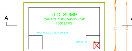
SUMP DETAIL
