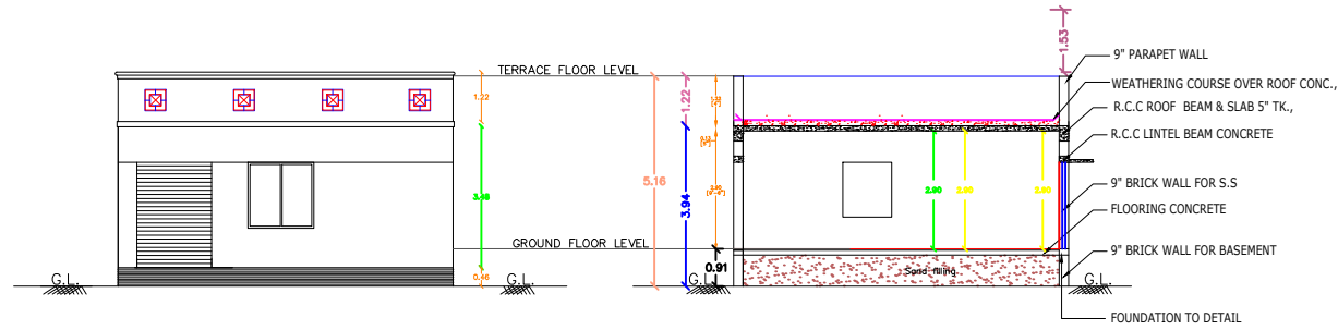
FRONT ELEVATION
