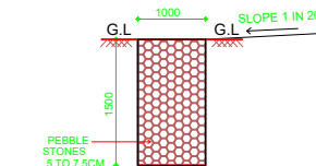
SECTION OF PEBBLE TRENCH SCALE : 1 : = 100
