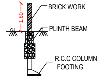
SECTION
