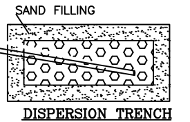
DISPERSION TRENCH
