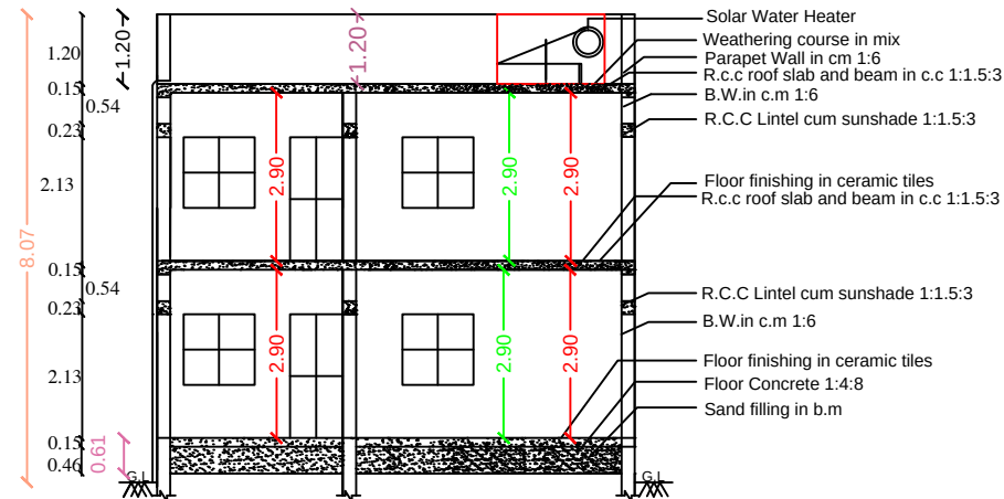
SECTION - "AB - CD"
