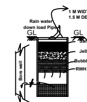
SEC. RAIN WATER HARVEST PIT
