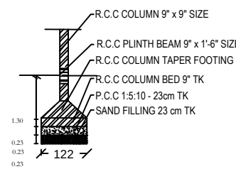
SECTION
