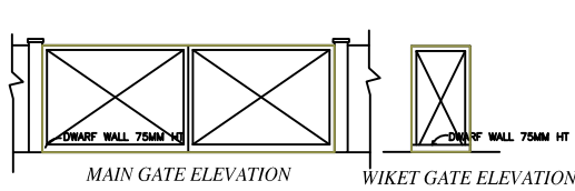
MAIN GATE ELEVATION
