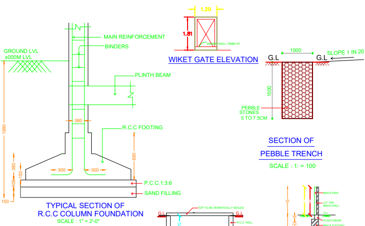
TYPICAL SECTION OF R.C.C COLUMN FOUNDATION
