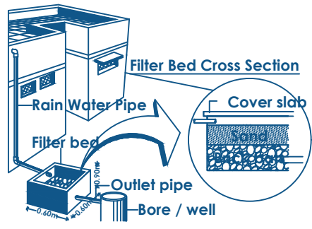
DETAILS OF RWH
