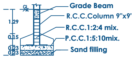
COLUMN DETAILS
