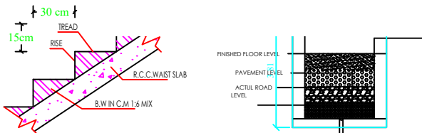
SECTION OF STAIRCASE
