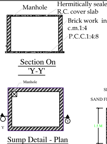
Sump Detail - Plan
