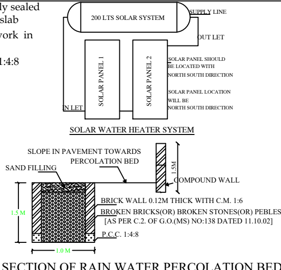
SECTION OF RAIN WATER PERCOLATION BED
