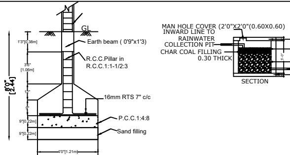
FOUNDATION DETAILS
