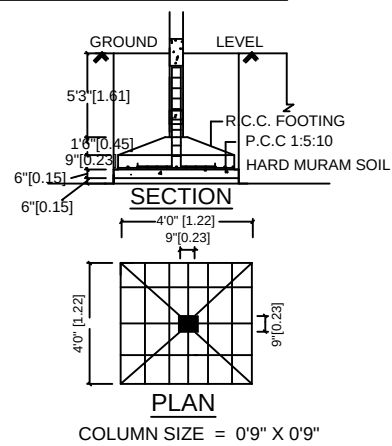
FOUNDATION DETAILS
