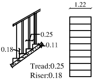
STAIRCASE DETAIL
