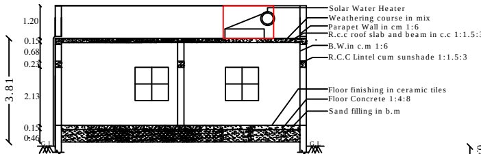
SECTION - "AB"
