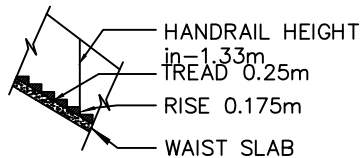
STAIRCASE DETAILS
