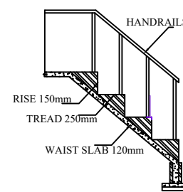
STAIRCASE DETAILS
