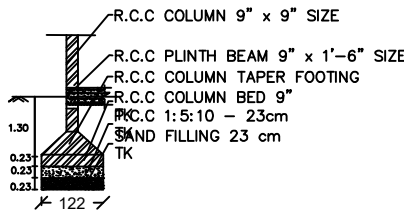
SECTION COLUMN DETAILS PLAN
