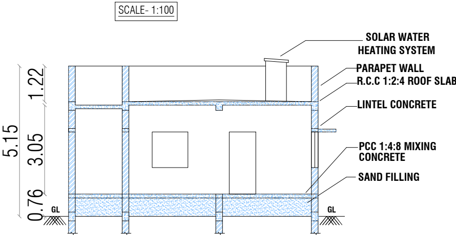
SECTION NO -"AB"
