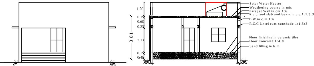
SECTION - "AB "
