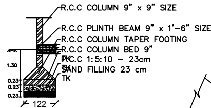
COLUMN DETAILS PLAN
