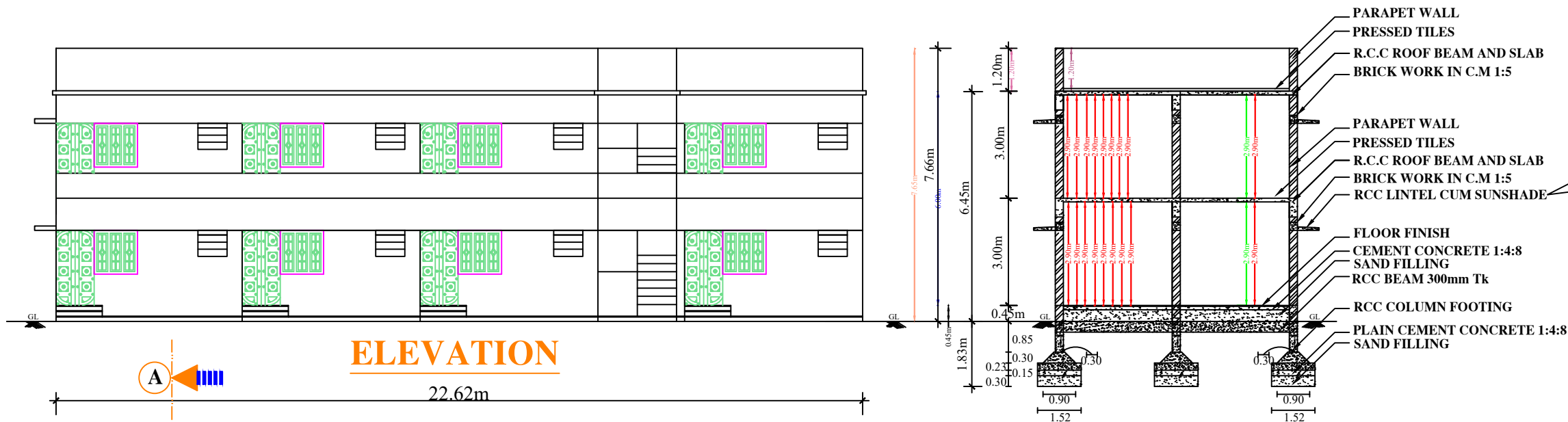
SECTION [A-A]
