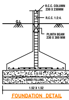
FOUNDATION DETAIL
