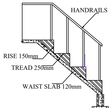
STAIRCASE DETAILS
