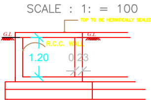
RWH SECTION (SAMPLE) RWHP CAPACITY_L = 2000LTRS
