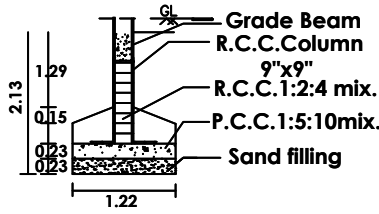
COLUMN DETAILS
