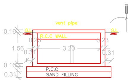
SECTION ON D-D
