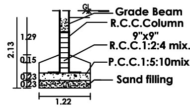
COLUMN DETAILS
