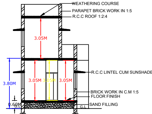
SECTION ON XX
