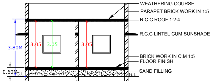
SECTION ON XX
