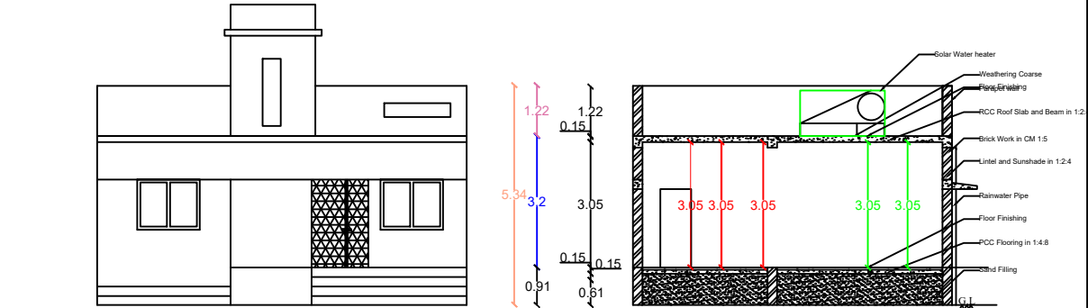
SECTION - "AB"
