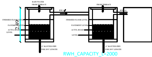
RWH_CAPACITY_L=2000
