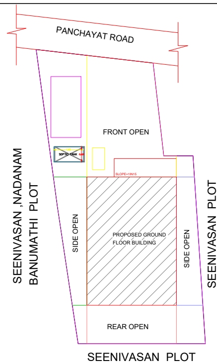
SITE PLAN SCALE:1:150
